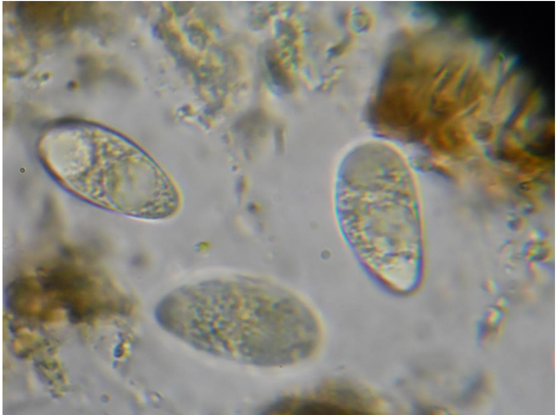
Spores 21-22 x 10-11 \mu\text{m}
