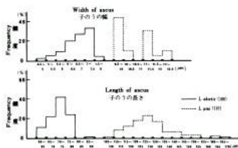
Fig.20. Histogram of length and width of ascus in 2 species of Lachnellula on Pinus (Total account of measured asci)
