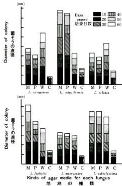
Fig. 7. Mycelial growth on various agar media
